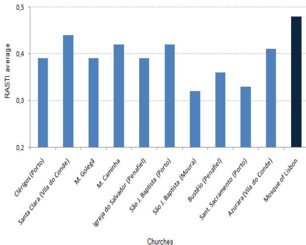
Figure 7 – RASTI average values (without SRS) in the Mosque of Lisbon and in the Portuguese Catholic churches with similar volume.
