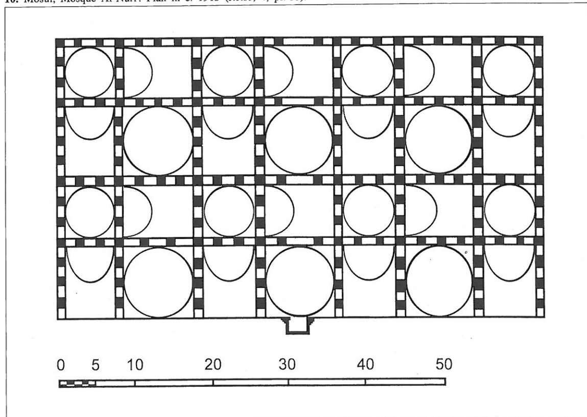
11. Mosul, Mosque Al-Nuri: Reconstruction of plan of first mosque. (Redrawn after Herzfeld in Reise , 4, fig. 237).
