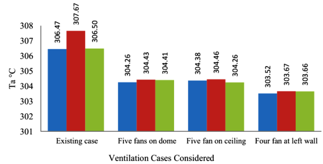
Figure 10 Plots of average air temperature in the east-, middle- and west-zone on a vertical (east-to-west) symmetrical plane.
