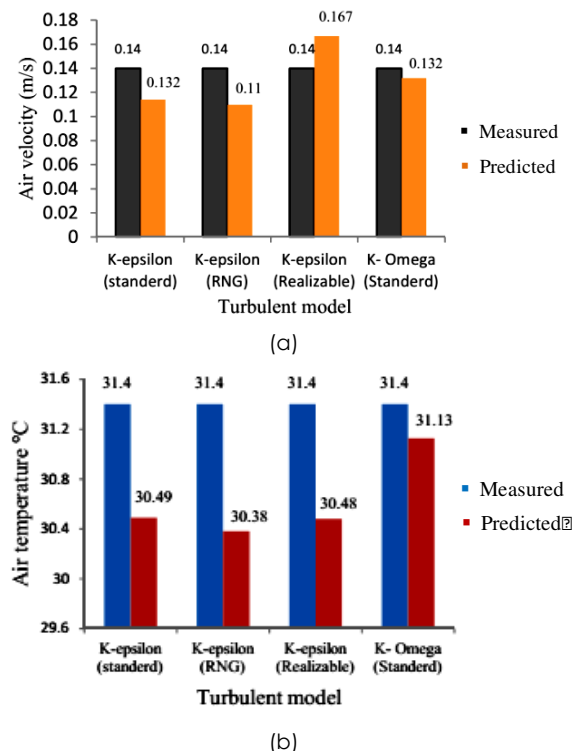
Figure 7 Comparison of (a) Airflow velocity, and (b) air temperature for various turbulent flow models with the corresponding measured values.
