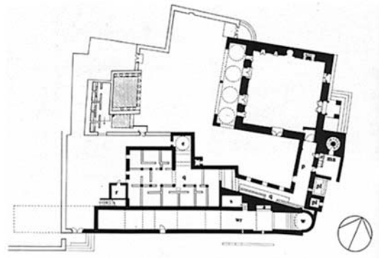
Figure 14. Sana'a, plan of Mosque of Talha[21]
