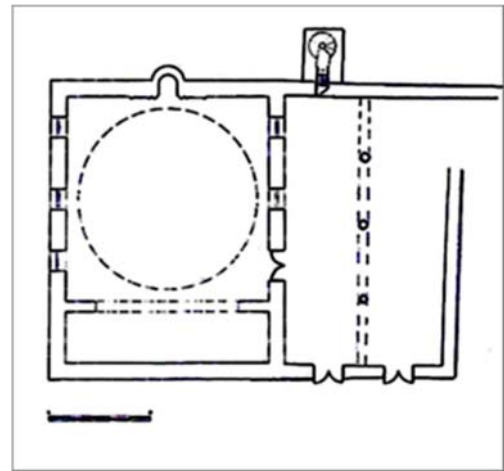
Figure 8. Sana'a, plan of Al-Muradiyya Mosque [18]
