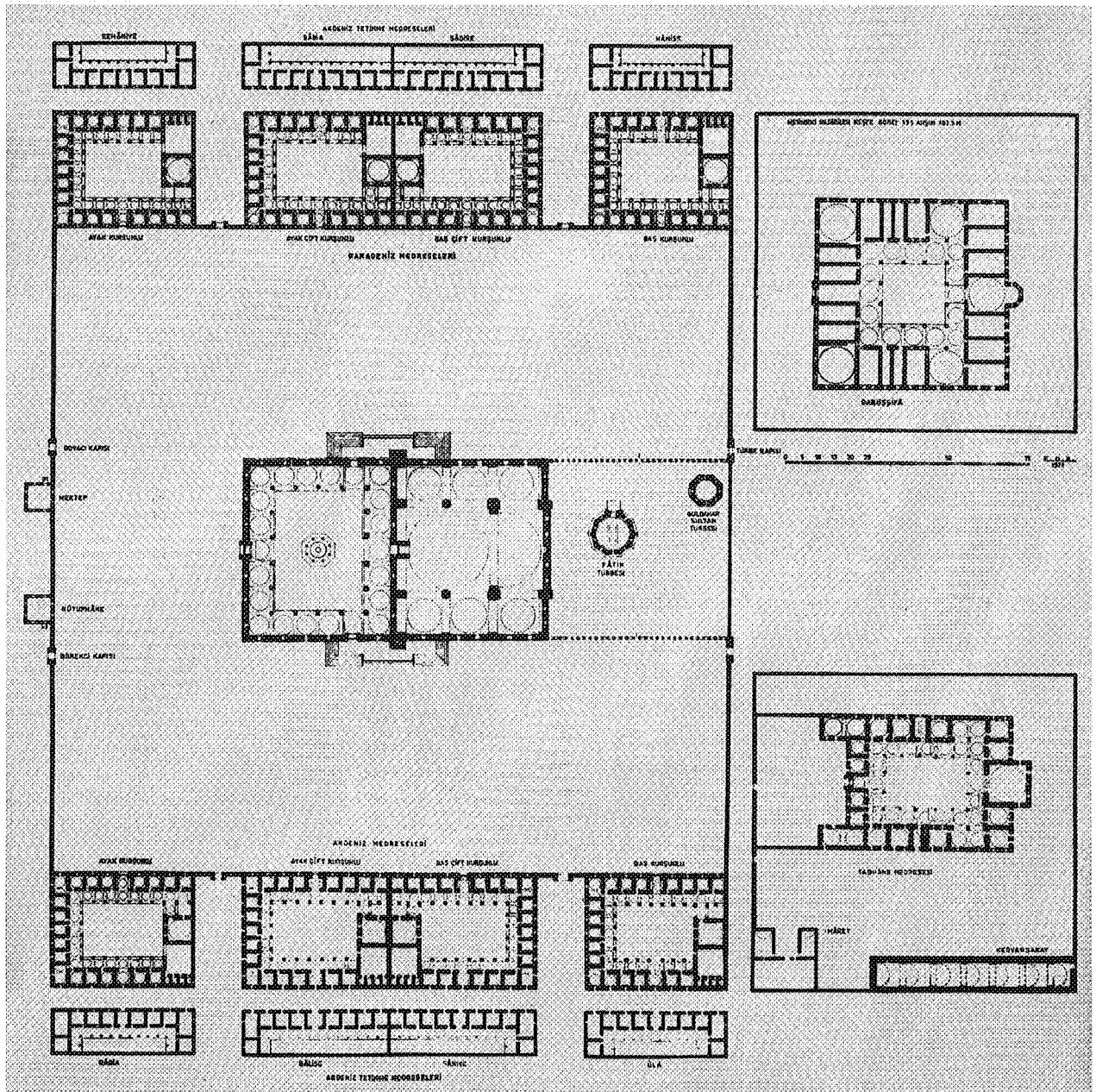
Plate 8. Istanbul. Mehmed II's complex. Plan from Ekrem Hakki Ayverdi, Osmanlı Mimarisinde Fatih Devri (855-886/1451-1481) (Istanbul, 1973), vol. 3.
